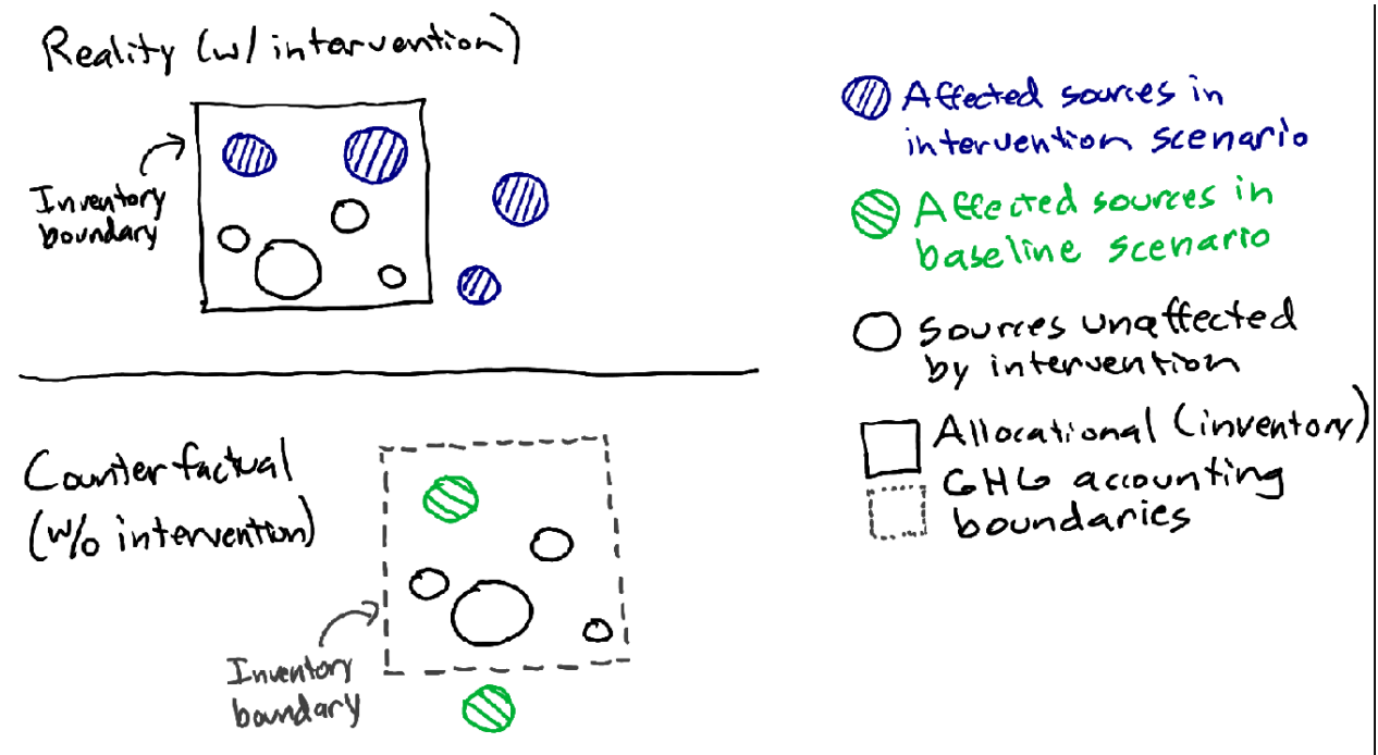
Figure 3. Illustration of boundary setting distinctions between allocational (inventory) and consequential (intervention) GHG accounting
